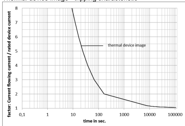
Thermal device image - tripping characteristic
