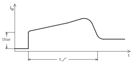
Diagram for start with voltage ramp
