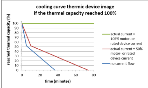
Thermal device image - cooling curve
